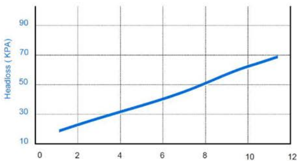
Specific air load of the OXYO™ - T65 membrane tube diffuser ( Nm 3 /h per running metre )
