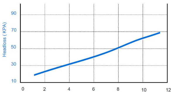
Specific air load of the OXYaero™ - T65 membrane tube diffuser ( Nm 3 /h per running metre )
